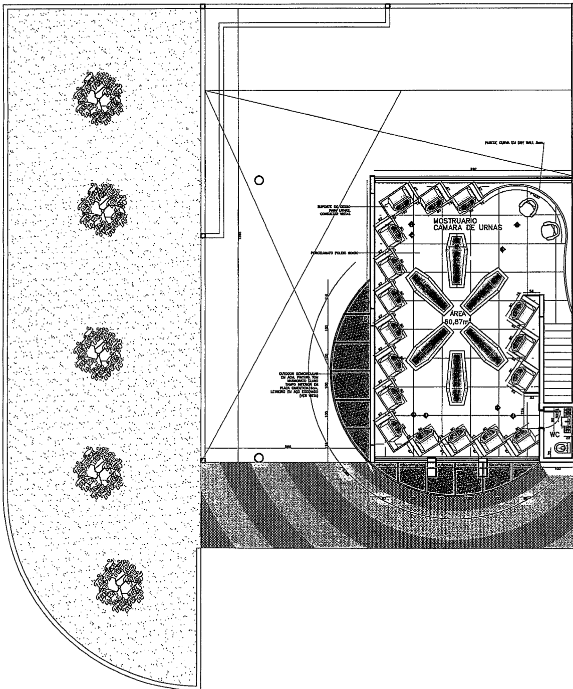
LAYOUT SUPERIOR Escala 1/50
